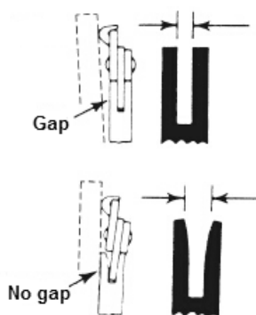
Chain tilts
